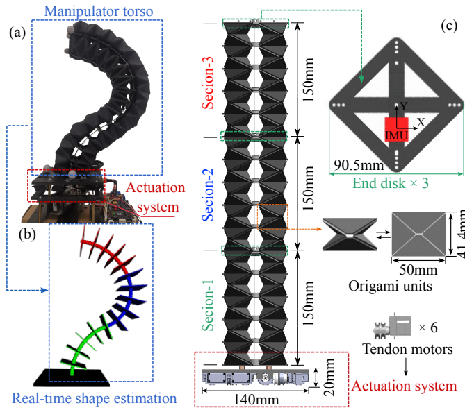
Fig. 1. (a) The authors develop the original prototype of a continuum manipulator with three continuum sections. (b) A virtual robot model based on the proposed shape estimation method is shown in the ROS-Rviz environment. (c) Mechanism details of the proposed continuum manipulator, including the torso, the end disks with IMUs, the actuation system with tendon motors, and origami units.
