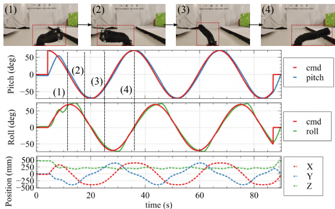
Fig. 6. System operation durability evaluation of the proposed manipulator by consecutively conducting the closed-loop attitude-tracking motion. The Roll and Pitch angles are derived from the attitude of the end-effector. “cmd” means the input command.
