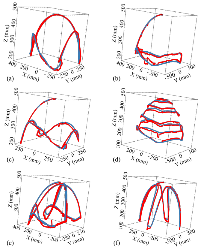
Fig. 8. Tip dynamic tracking results of our method (blue curves). Ground truth (red curves) are obtained by the motion capture system. (a) Trajectory with three waypoints. (b) Trajectory with four waypoints. (c) Circle trajectory. (d) Spiral trajectory. (e) Eight-shape trajectory. (f) Spark trajectory.
