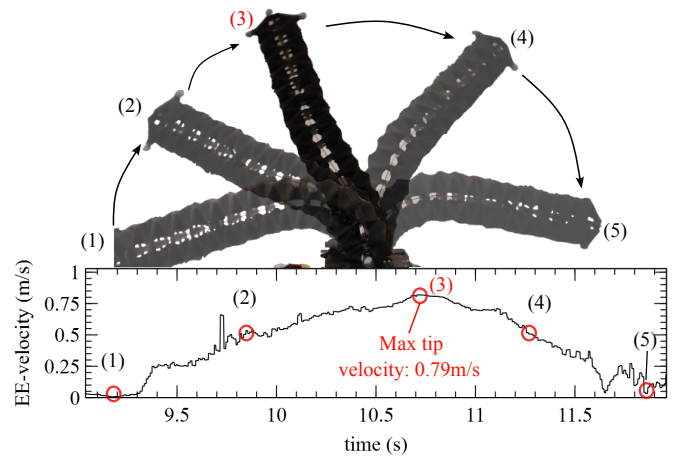
Fig. 5. Measurement of maximum tip velocity. (1-5) Five shape configurations during the fast swing motion. (3) The maximum tip velocity is 0.79 m/s.
