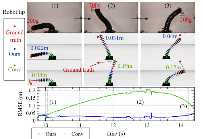
Fig. 11. Dynamic motion with a loading: 200 g. RMSE results of our method ("Ours") and the conventional method ("Conv") are presented.
