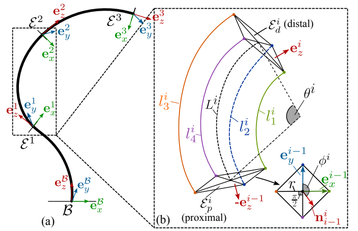
Fig. 2. Configuration space's description of the proposed continuum manipulator. (a) Overview of the whole configuration including key coordinate frames. (b) Single section's configuration including key numerical variables.
