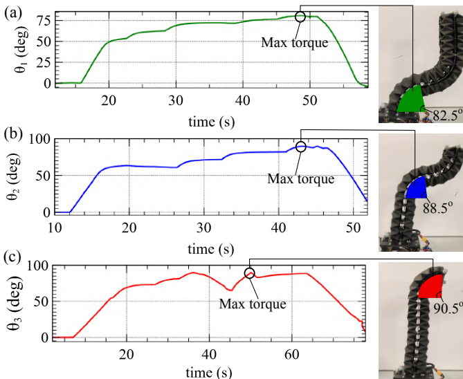
Fig. 3. Maximum bending angles of three sections by the IMUs' EKF, with actual shape situations of the continuum manipulator. (a) The first section: 82.5^\circ . (b) The second section: 88.5^\circ . (c) The third section: 90.5^\circ .
