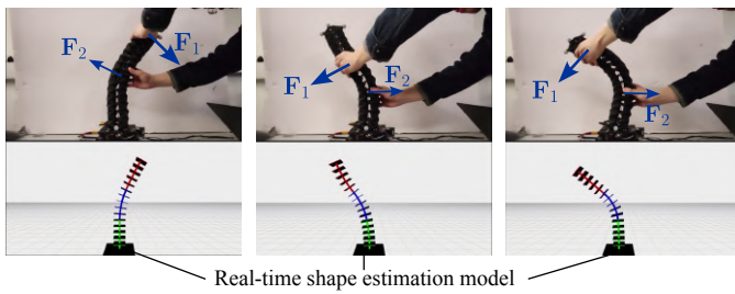
Fig. 9. Shape estimation by the proposed method under external intervention.
