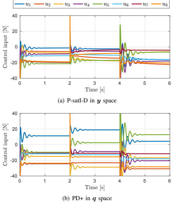
Fig. 6. Time evolution of the control inputs under the P-satI-D (24) in \mathbf{y} space and the PD+ (25) in \mathbf{q} space, respectively.
