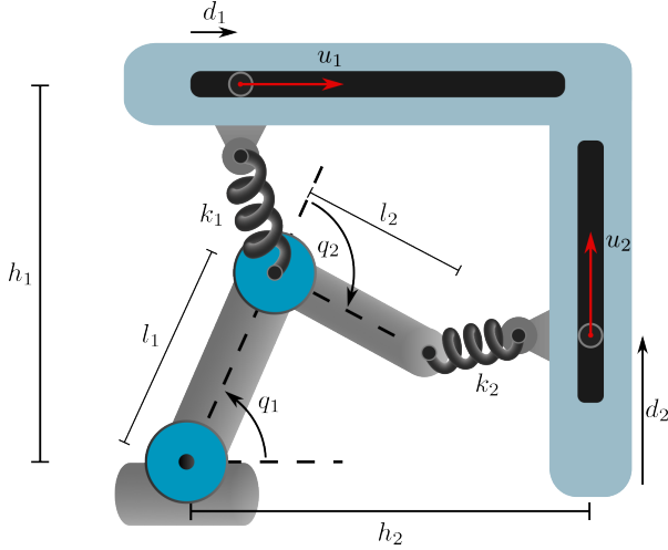
Fig. 3. A planar mechanism with two rotational joints having configuration \mathbf{q} \in \mathbb{S}^1 \times \mathbb{S}^1 . Positive (relative) rotations are counted counterclockwise. For i = 1, 2 , the force u_i actuates a cart coupled to the robot by a linear spring of stiffness k_i . The dynamics of the carts is negligible, and thus the forces \mathbf{u} act instantaneously on the mechanism.
