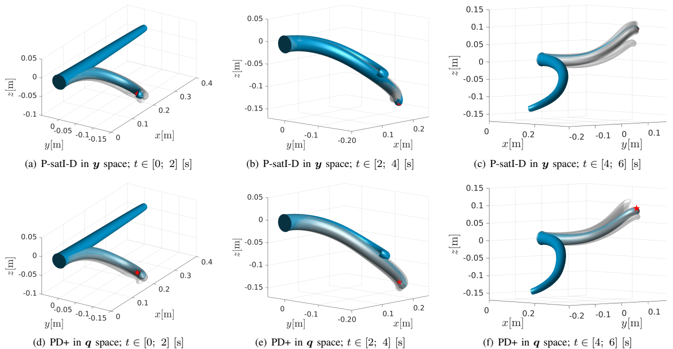
Fig. 8. Frame sequences of robot motion, divided in three time windows. Figs. (a)–(c) and (d)–(f) show the robot when controlled in the \mathbf{y} or \mathbf{q} coordinates using the laws (24) and (25), respectively. The initial and final configurations of each interval are shown in blue, while light gray shapes represent intermediate configurations. A red star indicates the constant target position of the end-effector.
