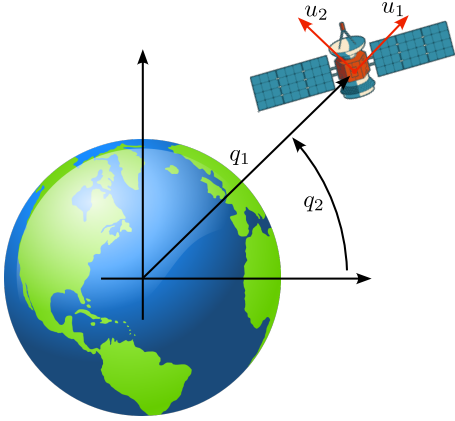
Fig. 2. A geostationary satellite actuated by a normal force u_1 and a tangential force u_2 . The body configuration is described by the distance q_1 from the Earth center and the angle q_2 with respect to the horizontal axis. Only the normal force is collocated because it performs work directly and only on q_1 .
