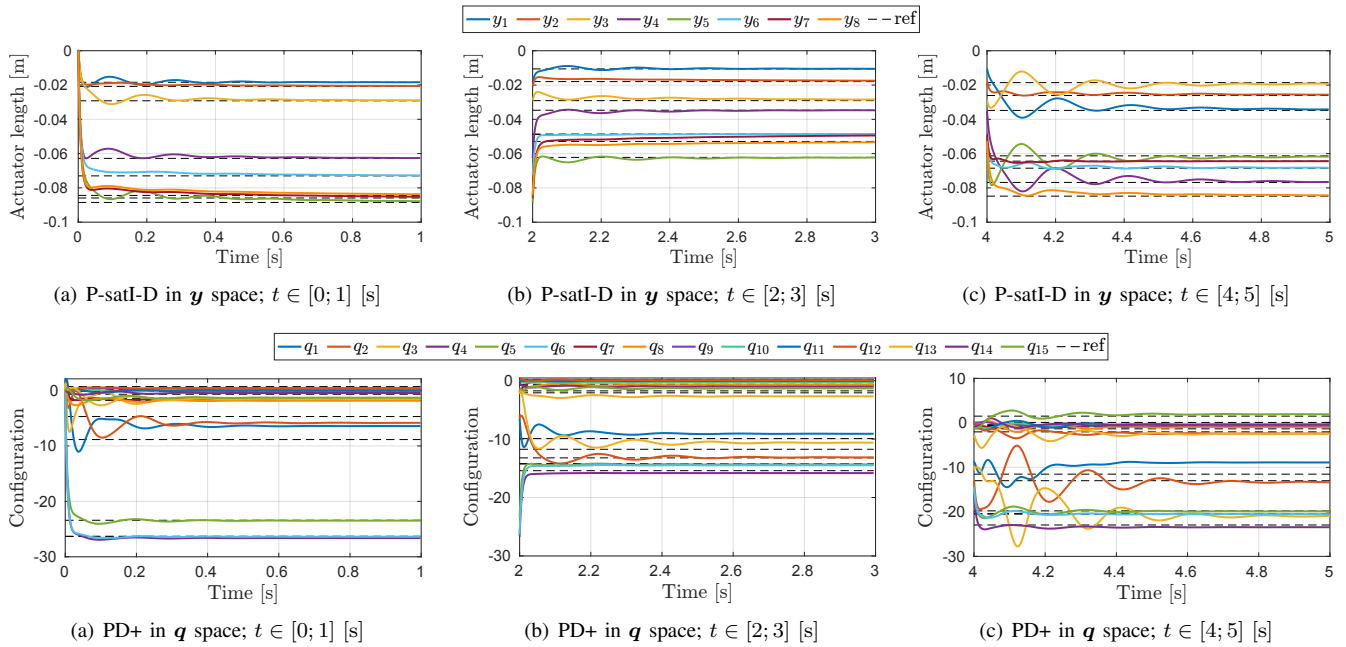
Fig. 7. Time evolutions of (a)–(c) actuator elongations and (d)–(f) configuration variables under the P-satI-D (24) in \mathbf{y} space and the PD+ (25) in \mathbf{q} space, respectively. The P-satI-D regulates the actuation coordinates to the desired target. On the other hand, the closed-loop system under the PD+ regulator is stable but has a steady-state error.
