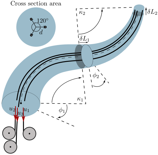
Fig. 5. A continuum soft robot discretized into two bodies. Under the piecewise constant curvature assumption, the configuration of each body is described by its curvature \kappa_i , bending angle \phi_i and elongation \delta L_i for i = 1, 2 . Three tendons run from the base to the tip, and spatial motion is obtained by applying a suitable cable tension \mathbf{u} \in \mathbb{R}^3 .
