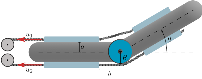
Fig. 4. A tendon-driven rotational joint having a single configuration variable q \in \mathbb{S}^1 . The cables tension u_1 and u_2 generate a torque at the joint.
