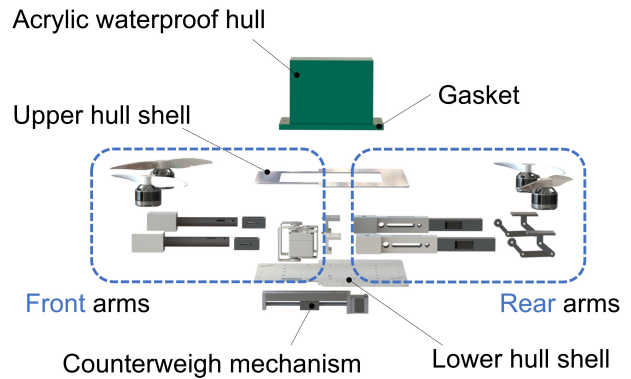
Fig. 2: Exploded view of the prototype design.
