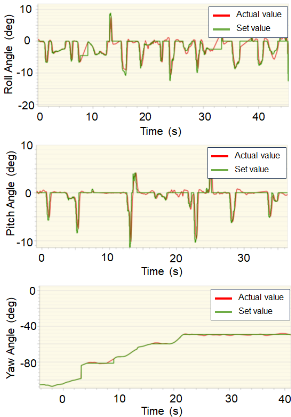
Fig. 9: Euler angles and respective set point angles of the vehicle over time as it conducts a flying maneuver in the field.
