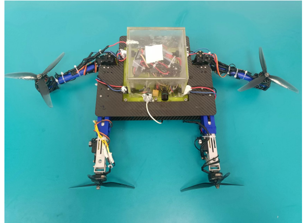
Fig. 1: Proposed multi-mode aerial-aquatic quadrotor vehicle with tilting mechanism.
