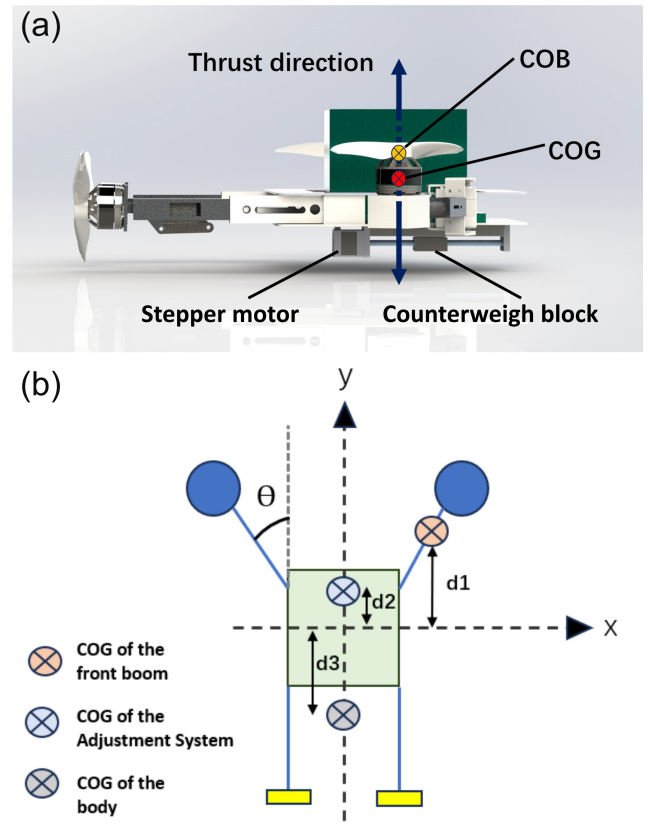
Fig. 5: Principle of center of gravity adjustment. (a) COG, COB, and thrust direction collinear; (b) the schematic diagram of gravity adjustment.
