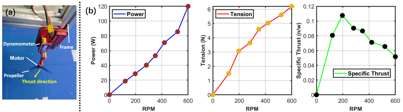
Fig. 7: The performance test of the propeller when actuated underwater. (a) Measurement setup; (b) results.
