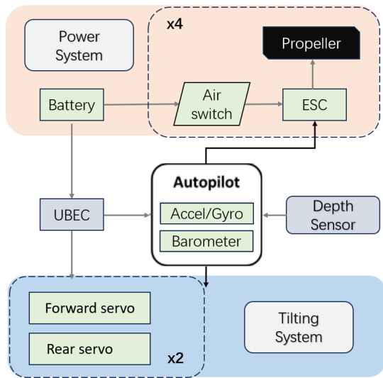
Fig. 6: Control structure of the designed quadrotor.
