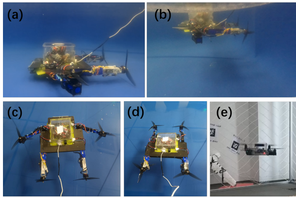
Fig. 8: Testing of the prototype from (a) diving to (b) floating, and transiting on the water surface from (c) water mode to (d) air mode, and (e) aerial flight.
