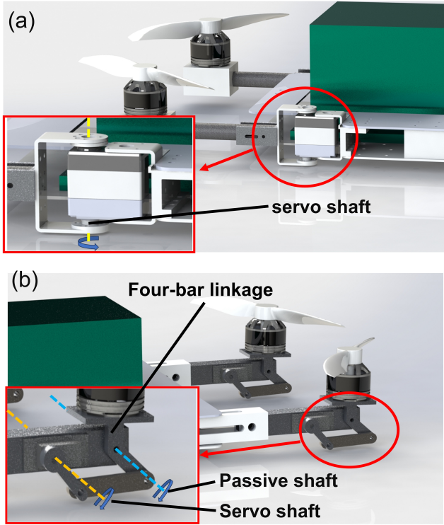
Fig. 4: Tilting mechanism. (a) Front tilting mechanism for arm rotation; (b) rear tilting mechanism for propeller rotation.
