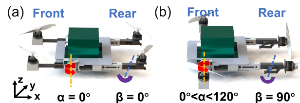
Fig. 3: Modes and corresponding joint angles of the vehicle for different environment propulsion. (a) Air mode; (b) water mode.
