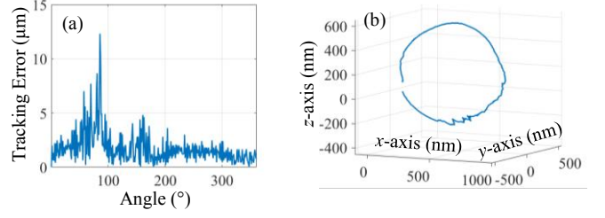
Fig. 7. (a) Tracking error on image plane during rotation with PID controller. (b) Real path of linear nanopositioners during in-situ rotation.
