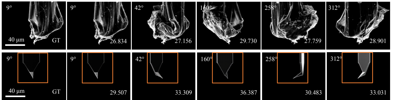
Fig. 8. Synthesized results and ground truth at different rotation angle for the two datasets. The presented images are respectively at angle of 9^\circ , 42^\circ , 160^\circ , 258^\circ , and 312^\circ . The first row is on dataset of a nanotube. The second row is on dataset of an AFM cantilever. The rectangles with orange border are the actual rendered region of 300 \times 300 pixels. All the data were captured at magnification of 1000. Peak Signal Ratio (PSNR) for each outcome is presented at the lower right corner and the corresponding rotation angle is at the upper left corner.
