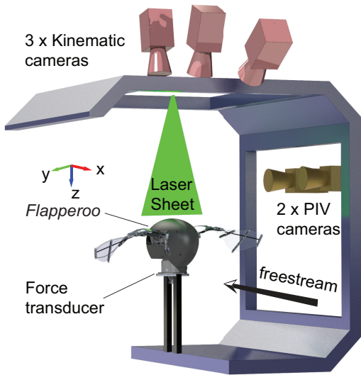
Fig. 3. The robot was tested in a closed-loop low turbulence level wind tunnel at Brown University [34].
