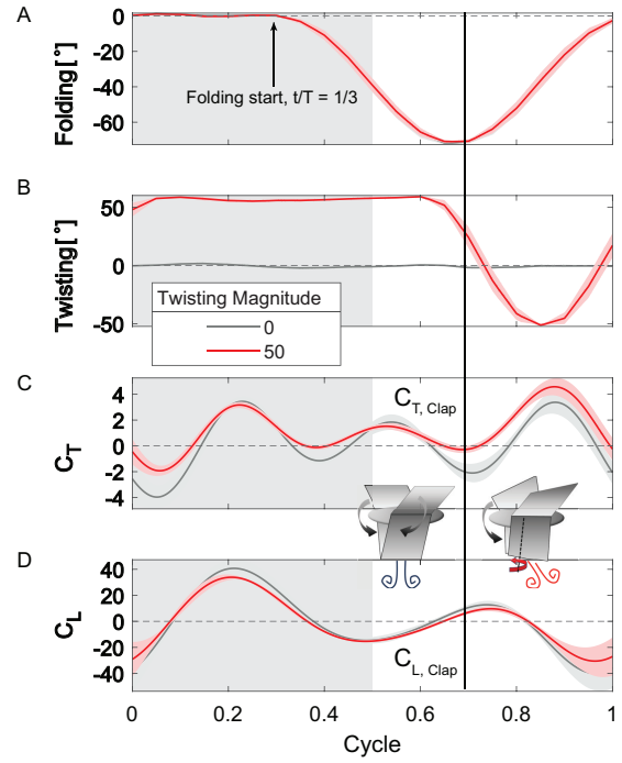
Fig. 4. Time series of the wing folding and twisting actuation, thrust and lift measurements. Note: the folding is already at maximum for twisting or non-twisting cases, and the wings would clap at the ventral side. The shaded area indicates the downstroke. The standard deviation calculated over 50 cycles is indicated by the bands around the signal. The black vertically running line indicates the moment of wing clapping, and the two cartoon insets illustrate the air jet produced and that is directed or “vectorized” with the wing twist.
