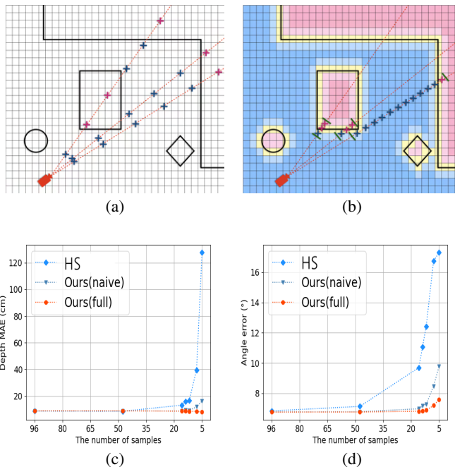
Fig. 1: (a): Baseline (hierarchical sampling). (b): Our method with near-far prediction. See the efficiency, accuracy, and robustness in the three rays, from left to right. Both (a) and (b) have an average of 6 samples per ray. Blue markers mean the model predicts SDF > 0 , and magenta markers SDF < 0 . Both (a) and (b) show only "coarse" samples for simplicity. (c-d): Trade-off between number of samples and accuracy. HS stands for Hierarchical Sampling, and "naive" is without adaptive sampling.
