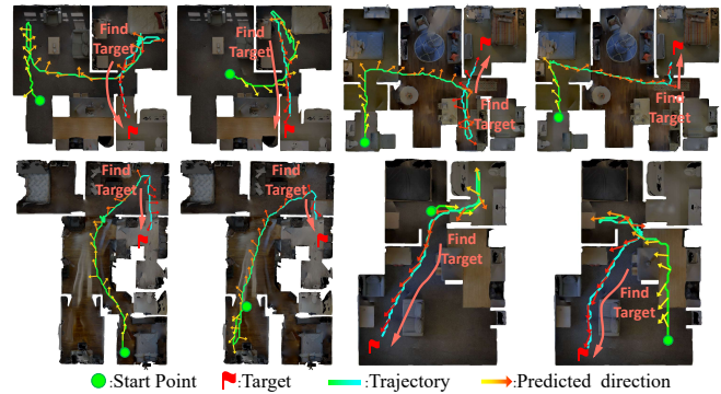
Fig. 5: Predicted results of the auxiliary task. The change in arrow color from yellow to red indicates the progress of navigation. During navigation tasks, auxiliary task accuracy steadily enhances, especially after observing the target.
