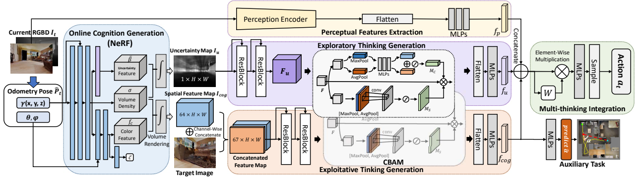
Fig. 3: The network structure of NUE. The overall framework first extracts real-time perceptual features and generates cognitive signals in NeRF. Subsequently, we compress the uncertainty map to generate uncertainty features and concatenate the spatial feature map with the target image in the channel dimension for spatial feature extraction. Finally, the features are concatenated and fed into an adaptive neural controller to generate the final navigation actions.
