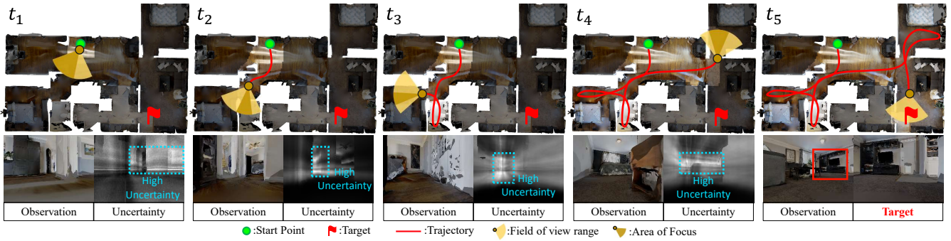
Fig. 4: Visualization examples of image-goal navigation. The visualized results showcase the behavioral logic of our model. Our model successfully utilizes uncertainty to explore the scene in the early stages of navigation, while also effectively leveraging cognitive information for navigation upon sighting the target.
