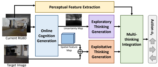
Fig. 2: The overall architecture of NUE. Firstly, real-time image input is used for online cognitive generation and perceptual feature extraction. Secondly, cognitive information is extracted to generate exploratory thinking and exploitative thinking. Eventually, multiple thinking is integrated, and navigational actions are generated.
