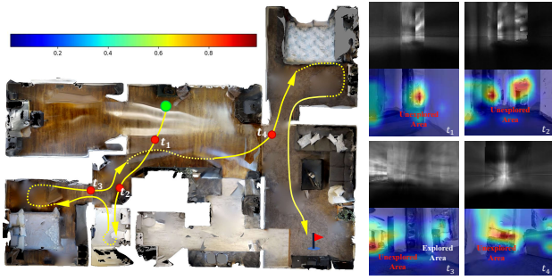
Fig. 6: Interpretation results of uncertainty extraction. The color in the image signifies the attention level of our uncertainty extraction structure on various regions. The top image in each pair shows the uncertainty map generated by NeRF, while the bottom image displays the gradient heatmap used for policy generation.
