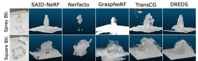
Fig. 7: Point clouds generated by methods tested. GraspNeRF does not use point clouds and its TSDF was converted for visualization
