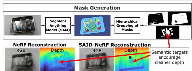
Fig. 3: Hierarchical semantic mask generation and its effects on transparent object reconstruction
