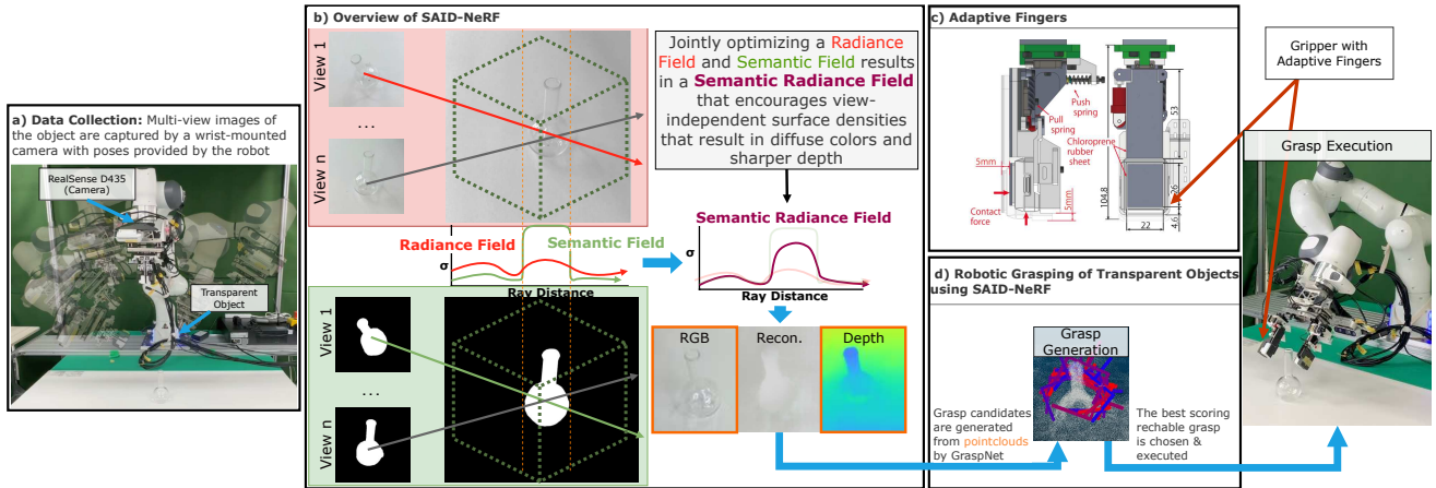
Fig. 1: Overview of the proposed system for robotic grasping using Segmentation-AIDed NeRF (SAID-NeRF) for depth estimation of transparent objects. SAID-NeRF uses Visual Foundation Models (VFM) for zero-shot segmentation to guide the reconstruction process
