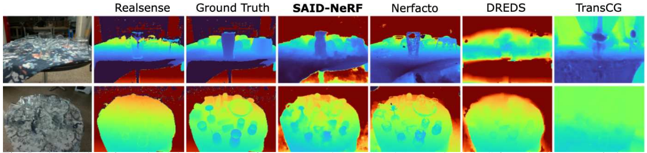
Fig. 5: Visualization of completed depth on scenes from “New Background” and “Heavy Occlusion” from the ClearPose [6] dataset
