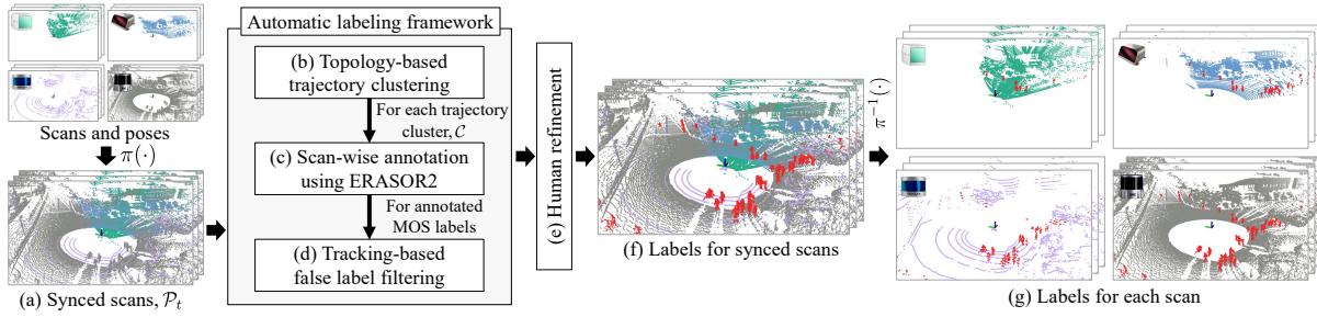
Fig. 3. Overview of our merging-and-splitting-based labeling framework. (a) Synchronization of the point clouds from the four LiDAR sensors at a software level. (b)-(d) Procedure of our proposed automatic labeling framework. (b) First, trajectories are segmented into multiple clusters. (c) For each trajectory cluster C , we apply an instance-aware static map building, ERASOR2 [15], that produces initial scan-wise annotated labels. (d) Tracking-based false label filtering is applied to reduce false positive and false negative MOS labels. (e) Next, these labels are manually corrected under human supervision. (f)-(g) Finally, the refined labels of synced scans are backpropagated to individual point clouds, which is denoted by \pi^{-1}(\cdot) . Red points indicate the annotated dynamic points (best viewed in color).
