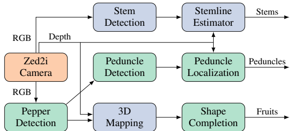
Fig. 6: Perception pipeline Hardware , Initial Mapping , Common . Stem detection and 3D mapping is done only during the initial mapping phase. Pepper and peduncle detection are carried out during initial mapping (Sec. IV-B) and fruit following (Sec. IV-D).
