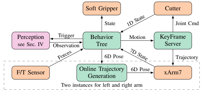
Fig. 7: Manipulation hard- and software pipeline. Behavior tree-based decisions control both xArm7s using motion primitives or online trajectory generation based on perception observations and sensor measurements. Colors correspond to categories (Hardware), (Manipulation), and (Perception).
