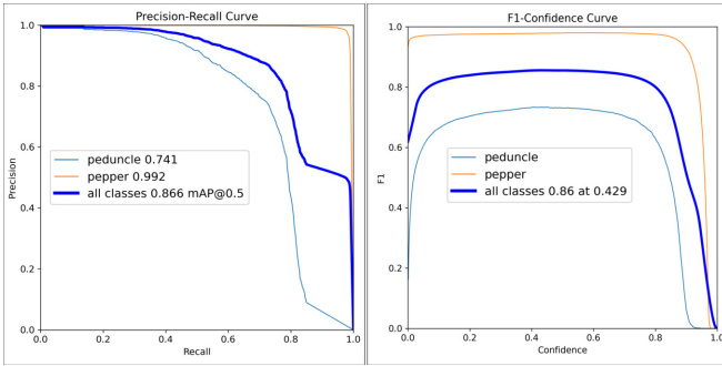
Fig. 10: Mask PR curve and F1 curve for peduncle detection in cropped image.
