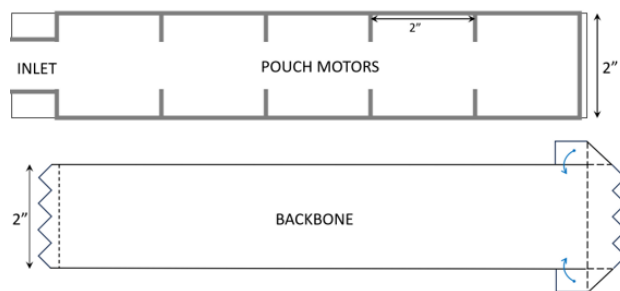
Fig. 8. The inchworm is composed of pouch motors and a flexible backbone. The pouch motors were laminated as shown along the gray bars. The backbone was made from 10 mil acrylic sheets, and folded 90^\circ along the long dashed lines and \sim 120^\circ along the short dashed lines. The pouches and backbone were attached using 0.25" strips of Gaffers tape.
