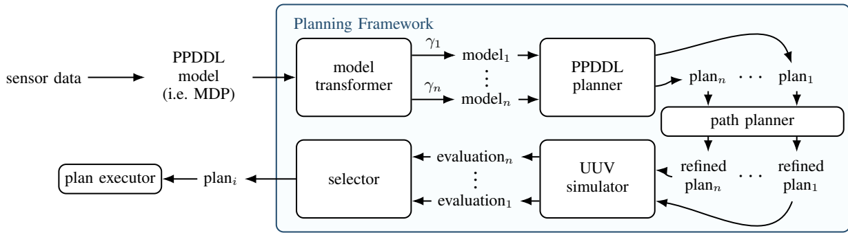
Fig. 3: Flow diagram of proposed method.
