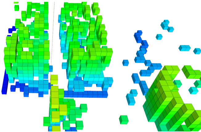
Fig. 6: A seabed OctoMap [17], using a low resolution (1000 samples with 0.5 resolution) sufficient for high-level planning. Each voxel represents a probability of occupancy.
