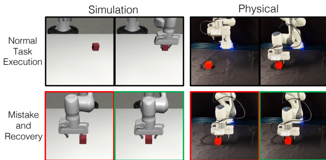
Fig. 4: Sim-to-Real. We evaluate sim-to-real transfer for a block grasping task with a Franka Panda robot. Similar to Figure 3 we show normal task execution, typical mistakes due to inaccurate object poses, and associated recovery for the simulation and real world environments. The results show that I-Gen can facilitate sim-to-real transfer of learned control policies, and that these policies retain robustness to erroneous perception.
