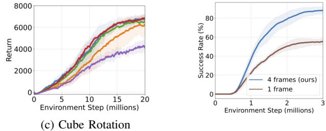
Fig. 7: Frame stacking ablation
