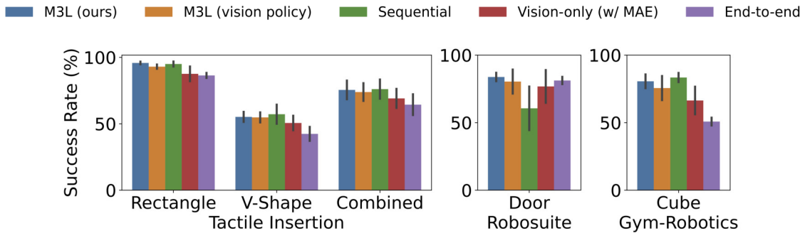
Fig. 5: Zero-shot generalization experiments on the three tasks. The bar plots show mean and standard error on 5 seeds, with 25 episodes run after training for the 4 last checkpoints on each seed.
