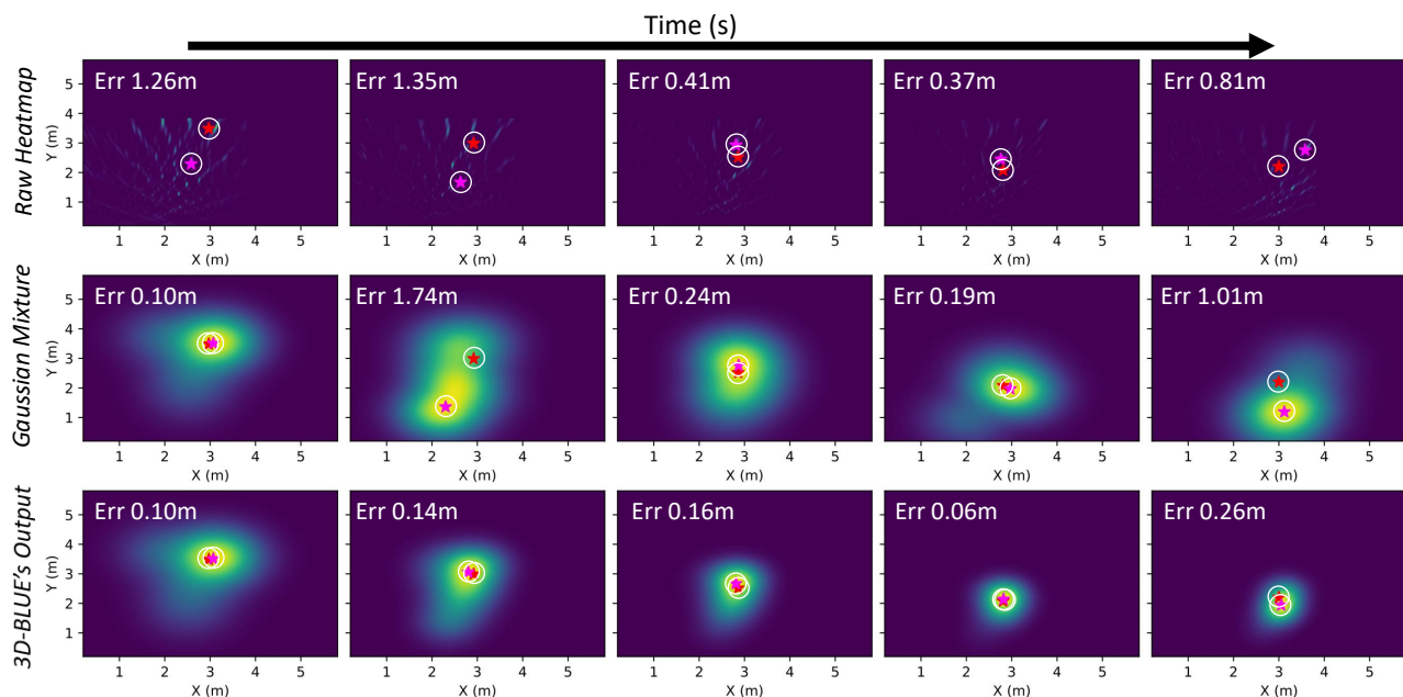
Fig. 7: 3D-BLUE's Particle Filter . The figure plots the probability distribution of the robot's location as a heatmap over 2D space, where yellow and navy blue indicate highest and lowest probabilities respectively. Rows 1, 2 and 3 show the heatmaps of P , P_n , and P_l respectively vs time.
