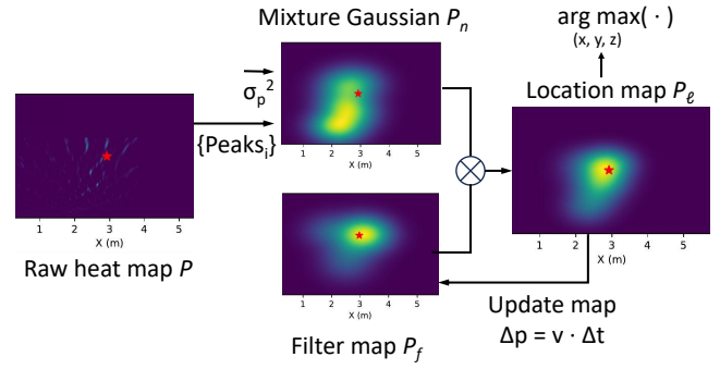
Fig. 6: Robust Location Estimation using 3D-BLUE's Particle Filter. Using the raw heat map P , 3D-BLUE generates a Gaussian mixture distribution P_n . It projects this distribution onto a filter map P_f and uses the output to obtain the location map P_l which it uses for location estimation. The location is updated with a motion model.
