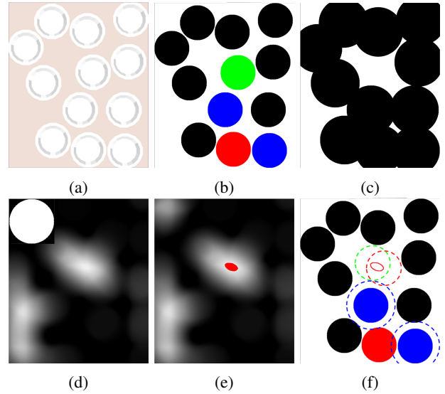
Fig. 5: (a) Current environment. (b) Current image. Red is the current target object. Blue is the remaining obstacle in the sequence. Green is the current obstacle in the sequence. (c) Binary image extended by r_g in the current image. (d) Mask image and result of the convolution with the binary image. (e) The image emphasizing areas that exceed the threshold. (f) The final selected image. The red dashed circle is the original obstacle position. The blue dashed circle is the area expanded by r_g around the obstacles in the sequence. The green dashed circle is the selected relocation position.
