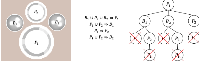
(b) An example where a relocation plan does not exist; In the search tree started from the target P_1 , all nodes are removed due to duplication in the path, leaving no more nodes to explore.
