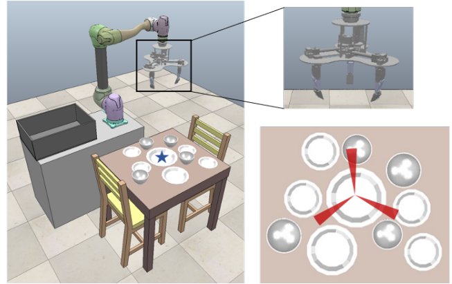
Fig. 1: Left: Table-clearing robot with 3-finger gripper. The table is densely filled with dishes. The target dish (blue star) is not graspable without rearranging the surrounding dishes. Right: An example of a target's local obstacle set, which collides with the gripper (red region). If the ones in the set are also not graspable, then additional obstacles must be relocated in order to make them graspable.
