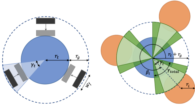
(a) The angle occupied by a finger denoted as \gamma_t , when grasping the target with a radius of r_t using 3-finger gripper. (b) The angle occupied by object i denoted as \gamma_i and the angle \gamma_{total} , which is expanded by the gripper.
