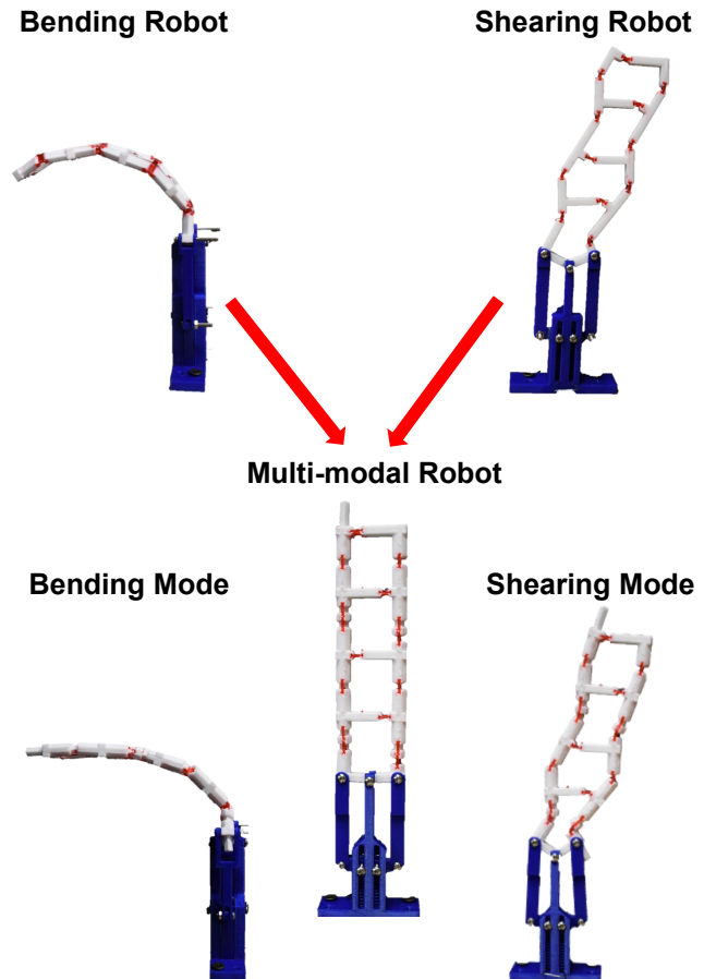
Fig. 1: In this work, the mechanical properties of two separate metamaterial robots are combined to create a multi-modal innovation which exhibits both behaviors in a single design.
