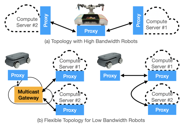
Fig. 4: Flexible Topology for Different Bandwidth of Robots (a) Since FogROS2-FT sends replicated requests to multiple cloud machines, it demands more network bandwidth than conventional cloud-robotics deployments. (b) FogROS2-FT allows flexible topology so that low-bandwidth robot can leverage cloud machines with higher bandwidth to forward to replicated services. One can either use dedicated gateway machine (left) or existing compute servers (right).
