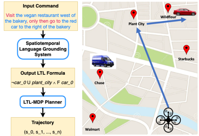
Fig. 2: An example of an input spatiotemporal navigation command whose spatial and temporal components are highlighted in blue and red, respectively, an output LTL formula whose propositions are grounded to physical landmarks, and an execution trajectory in the environment.
