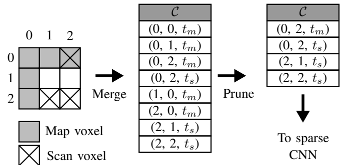
Fig. 3: Our method prunes map voxels without scan correspondence, significantly improving performance by eliminating unnecessary voxels. In this example, the map depicts a wall corner, and the illustrated scan voxels reveal the occlusion of some map voxels caused by an obstacle. We show the resulting voxel coordinates \mathcal{C} before and after pruning and indicate the map and scan timestamps as t_m and t_s , respectively.
