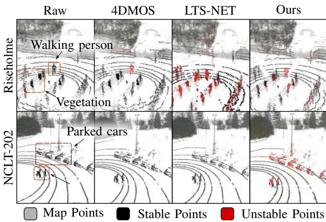
Fig. 5: Comparison of the generalization ability of our method to multiple baselines. Riseholme is recorded in an agricultural environment with walking persons and changing vegetation whereas NCLT is a parking lot with parked cars.
