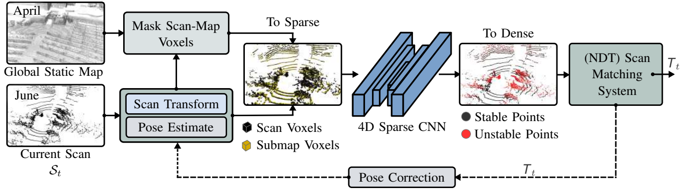
Fig. 2: An overview of our method: Initially, we transform the scan using an initial pose estimate. Next, we voxelize both scan and map points and extract overlapping map voxels, i.e. submap voxels. Both the scan and map voxels are represented as a 4D sparse tensor, with the fourth dimension denoting time t . We then apply sparse 4D convolutions on a joint sparse voxel grid that encompasses both the scan and submap points, leading to the prediction of long-term stability scores for the scan points.
