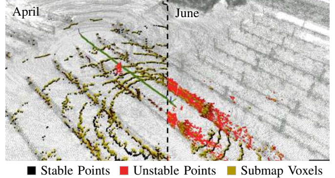
Fig. 1: Our method segments stable and unstable points in 3D LiDAR scans exploiting the discrepancy of scan voxels and overlapping map voxels (highlighted as submap voxels). We showcase two LiDAR scans captured during separate localization sessions within an outdoor vineyard. The scan on the left depicts the vineyard state in April, while the scan on the right reveals environmental changes in plant growth in June.
