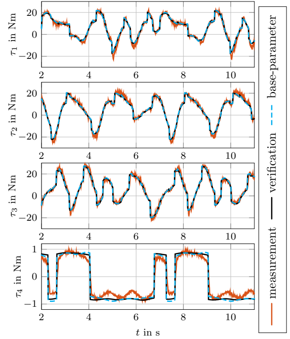
Fig. 7. Motor torques \boldsymbol{\tau} for the verification trajectory. The root mean squared (RMS) error of the base-parameter identification \mathbf{e}_{\text{RMS}}(\mathbf{p}_{\text{B}}) = [2.0 \ 1.8 \ 2.2 \ 0.25] \text{ Nm} is close to the \mathbf{e}_{\text{RMS}}(\mathbf{p}_{\text{Ident}}) = [2.0 \ 1.7 \ 2.2 \ 0.20] \text{ Nm} of the parameter \mathbf{p}_{\text{Ident}} identified with the proposed method.
