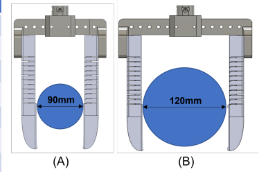
Fig. 14. On the left, items of the pick-and-place demonstration and their corresponding weight are listed. On the right, the two fixed gripping widths (A&B) of the MERA-gripper adopted in Fig. 15 are illustrated.
