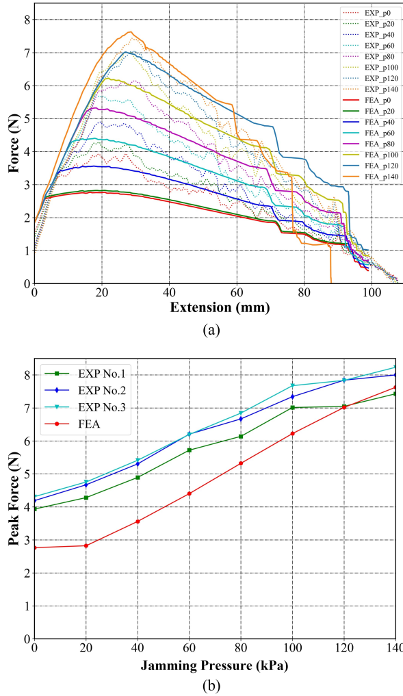
Fig. 8. (a) FEA simulation results VS experimental results (experiment No.1) and (b) The simulated peak contact force at different applied pressures in the jamming channel.
