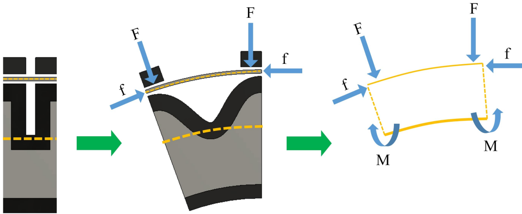
Fig. 4. A jamming unit (left) has two neutral bending axes at SSS and MERA respectively. Distance between the axes is fixed by the normal force provided by the restraining frame. Upon actuation (middle), the SSS goes through a sliding and pure bending motion since frictional force, f , is close to 0. In a jammed state (right), sufficient frictional force is present, f , to counter the torque M created by the load and depressurization.
