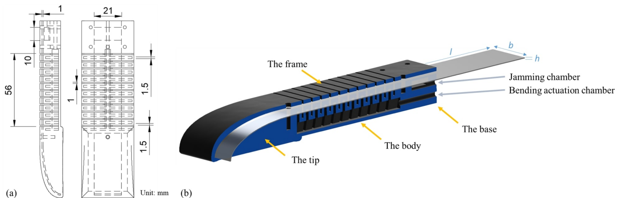
Fig. 2. (a) Internal dimensions of the variable stiffness actuator (b) A schematic of the components within the actuator
