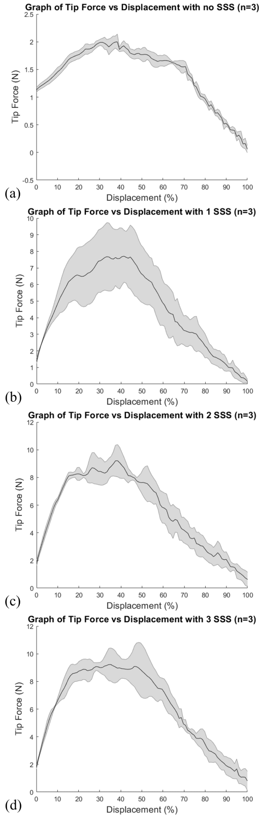
Fig. 11. Tip force with respect to cylinder displacement at 140kPa jamming pressure using the large cylinder (75mm in diameter) with (a)0 SSS, (b)1 SSS, (c)2 SSS, and (d)3 SSS installed in the MERA respectively. 3 repetitions (n=3) are conducted per experimental run.
