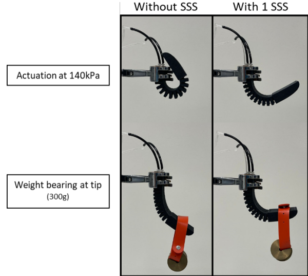
Fig. 1. With the reinforcement of the SSS, the metal-endoskeleton-reinforced actuator (MERA) proposed in this research could possess a higher stiffness that enables it to handle the same payload of 300g more stably.
