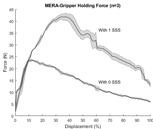
Fig. 13. The holding force of the MERA-Gripper measured by the experimental setup in Fig. 10. 3 repetitions ( n=3 ) are conducted per experimental run. Apparent advantages in payload and gripping stability were observed from the profile of the MERA with the jamming function on.
