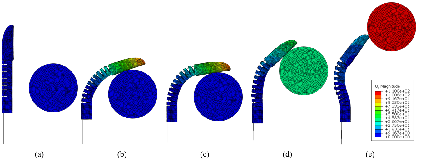
Fig. 6. Finite element simulation results of the actuation process and the interactions between the actuator and the moving cylinder. (a) The initial state of the actuator with a SSS inserted (b) The final state of the actuator after applying pressure in the main channel (c) The final state of the actuator after applying pressure in the jamming channel (d) The intermediate state of the actuator while the cylinder is moving upwards (e) The final state of the actuator when the cylinder is leaving the contact region.
