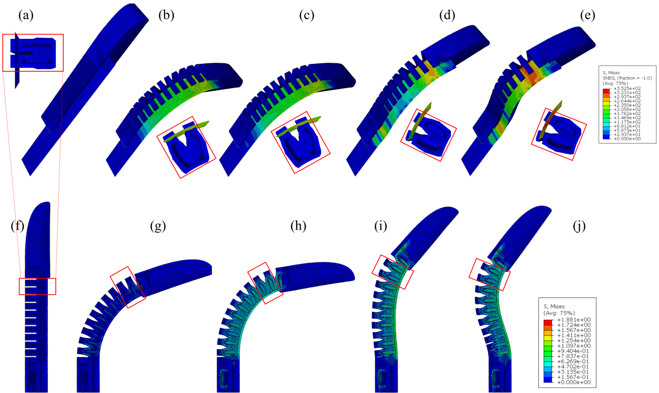
Fig. 7. FE simulation results of the stress distribution within the actuator and the SSS. (a-e) give the Mises stress evolution for both the finger and SSS, showing that SSS is bearing most of the stress induced by the system. (f-j) show the Mises stress distribution within the finger only, indicating that the stress level within the finger is much lower than that in the SSS. The insets in (a-e) are enlarged views of two units within the red boxes shown in (f-j). (a,f) Initial state (b,g) Final state of the actuator after applying pressure in the main channel (c,h) Final state of the actuator after applying pressure in the jamming channel (d,i) Middle state of the actuator when the cylinder is moving upwards (e,j) Final state of the actuator when the cylinder is leaving the contact region.
