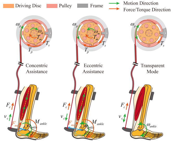
Fig. 2. Synergy mechanisms between the proposed actuation and the human muscle (taking soleus as an example). In assistive modes, the proposed actuation cooperates with the human muscle and reduces muscle activation by applying proper assistive force in parallel with the corresponding muscle–tendon system. In the transparent mode, the interaction torque between the device and the human fully depends on the pretension level of the torsion spring. In this figure, F_{\text{mu}} is the muscle force generated by the soleus, and L_{\text{mu}} symbolizes the moment arm of the muscle force relative to the CoR of the ankle joint. L_{\text{exo}} refers to the moment arm of the cable force generated by the actuation system. \omega_{\text{ankle}} and M_{\text{ankle}} represent the angular velocity and the moment of the human ankle, respectively.
