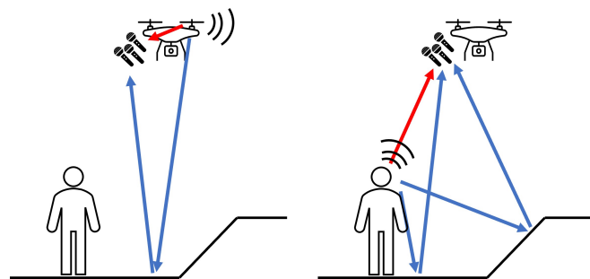
Fig. 2. Illustration of ego-noise and a human's voice propagation paths towards the microphone array, emphasizing direct sound paths in red and reflected sound paths in blue.
