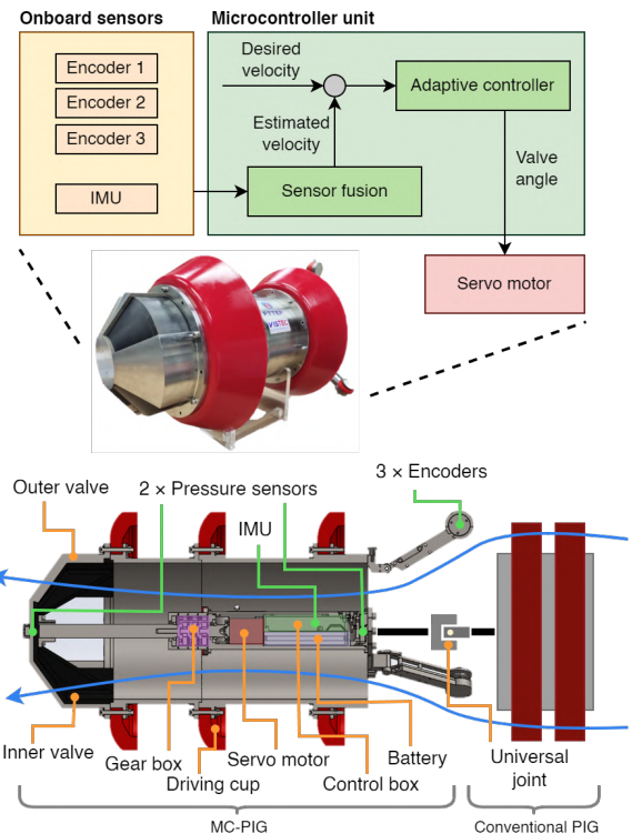
Fig. 1: A system overview of MC-PIG. The block diagram shows the EKF-based sensor fusion for speed estimation and adaptive PD control. The cross-section view demonstrates the key hardware components of MC-PIG. Blue arrows display the flow direction through MC-PIG.
