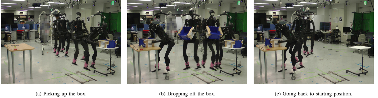
Fig. 6: Full loco-manipulation cycle by automatically switching policies online. The support crane has been partially edited out for visibility purpose.
